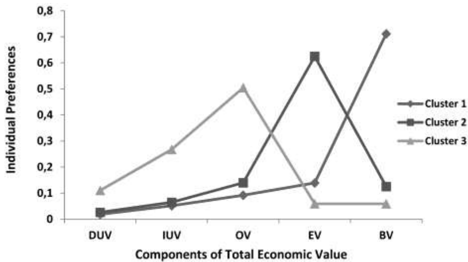
Fig. 2 Cluster profiles based on the medians. Source: Own elaboration
